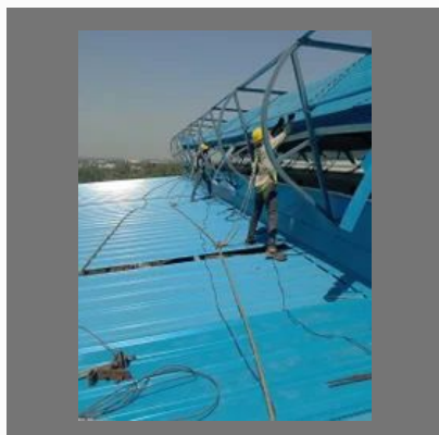
Industrial Ridge Ventilation System
